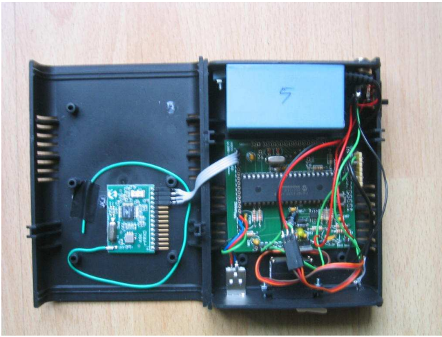
Figure 2: The NASCIO: the sensor/actuator board used for Schwelle II. The box shown is an actuator for moving and lighting electro-luminescent wire.
